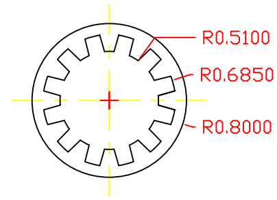
Lock Washer
