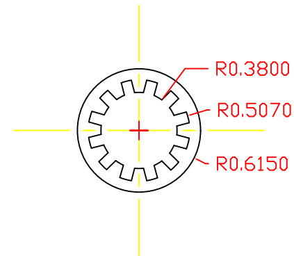
Lock Washer
