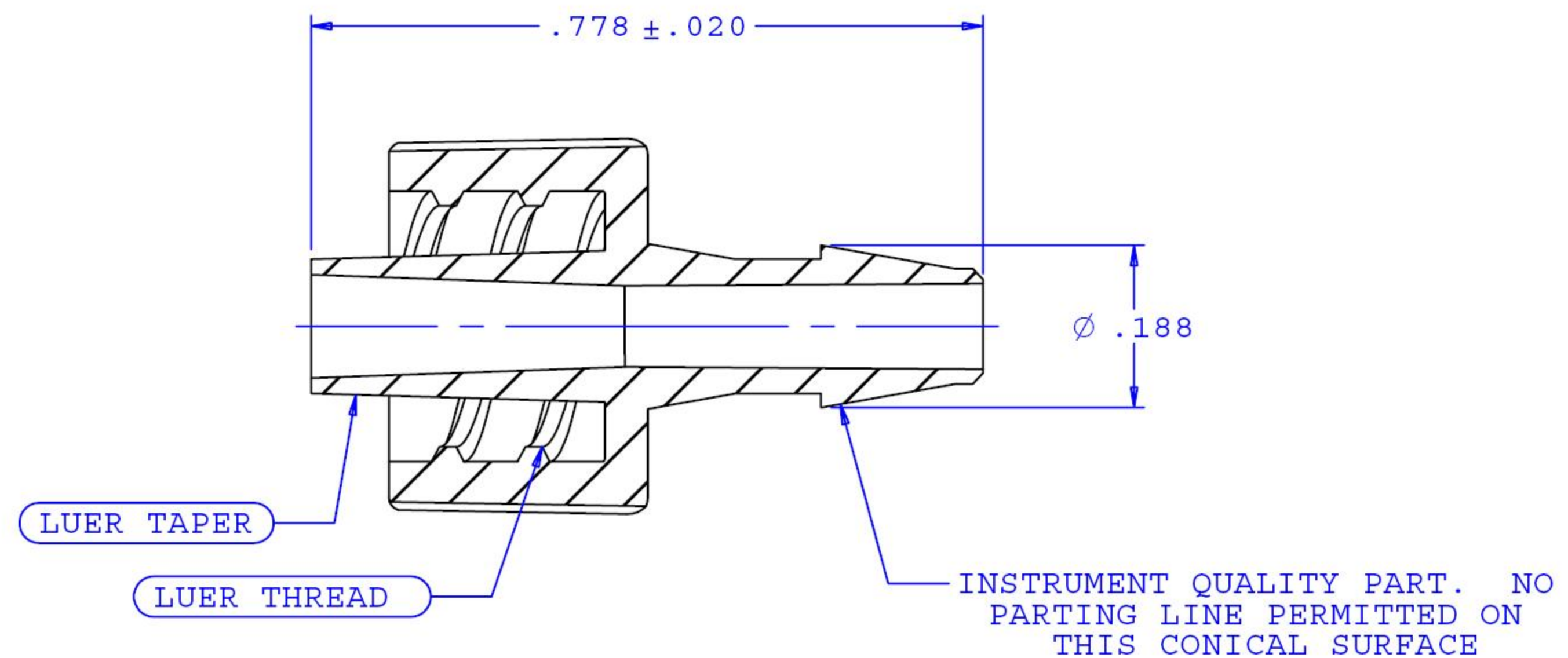
SECTION B-B
